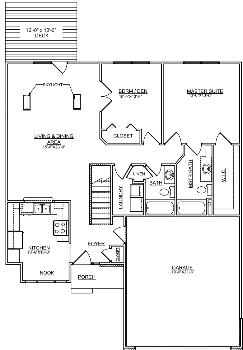
MAIN FLOOR 1218 SQUARE FEET
